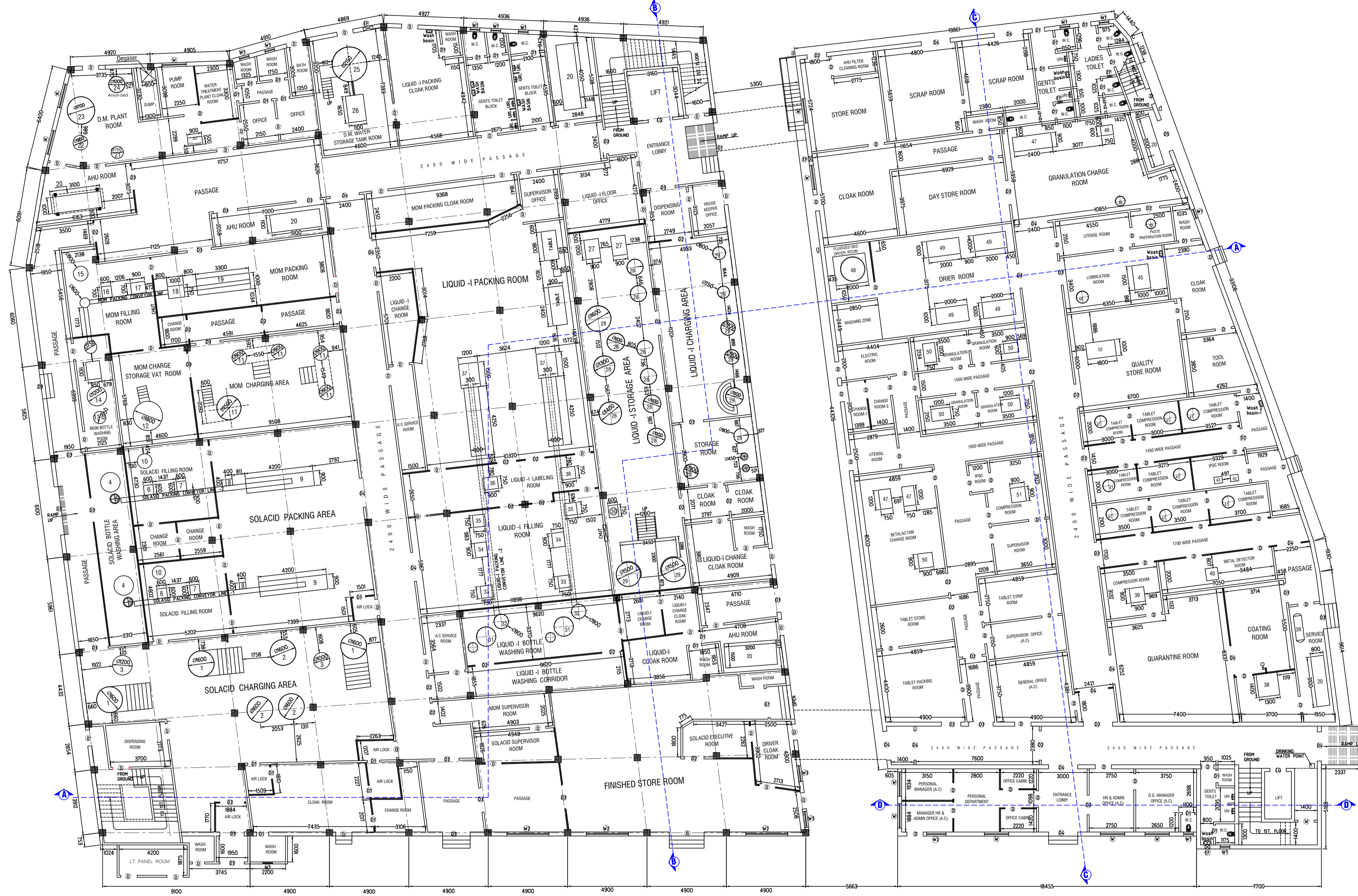
GROUND FLOOR LAYOUT PLAN OF SITE PLAN BLOCK NO - A & B (SCALE-1:100)
