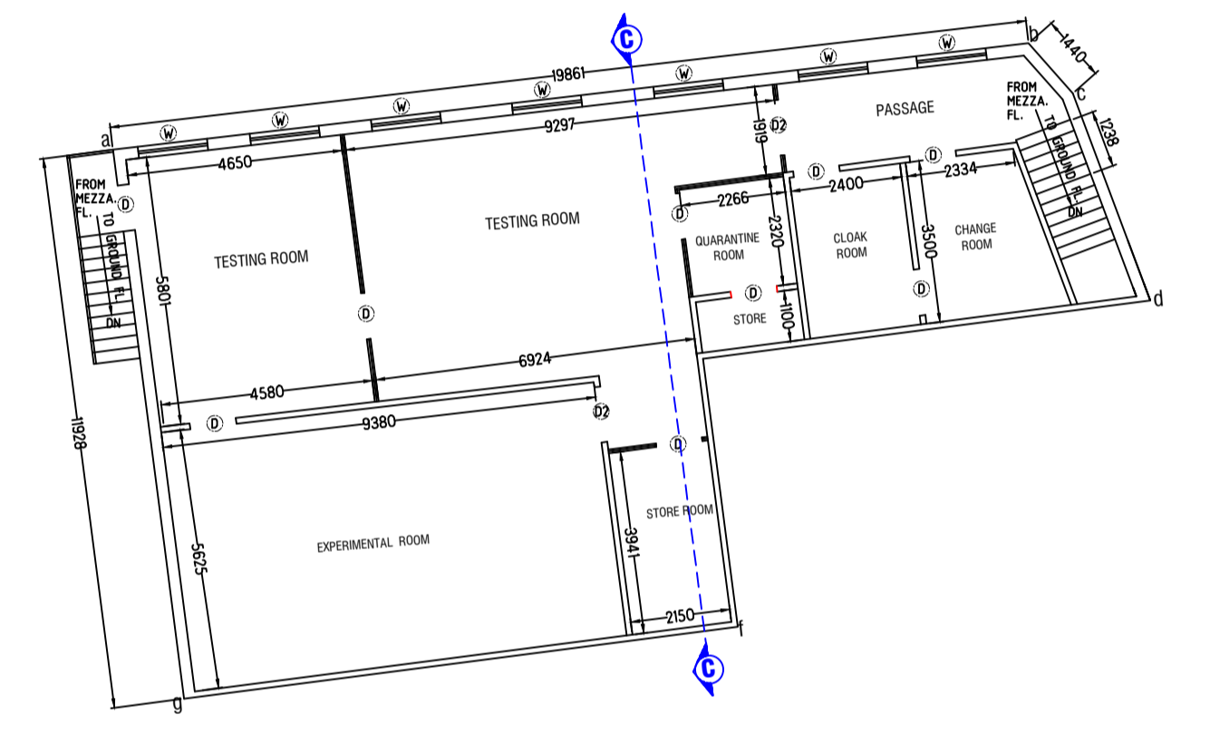
MEZZANINE FLOOR PLAN (a,b,c,d,e,f,g,a PORTION) SCALE-1:100
